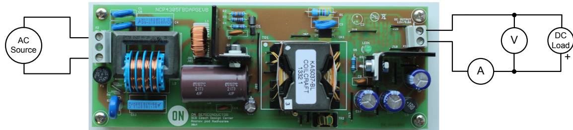
Figure 1: Test Setup
