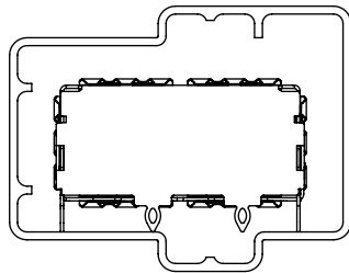
QSFPC-PF-01 (SEE NOTES 3 & 6)
