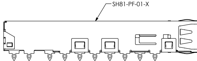
FIG 4 QSFP-CF-01-F SHOWN (NOT RELEASED) (SAME AS FIG 1, EXCEPT AS SHOWN) (SEE NOTE 6)
