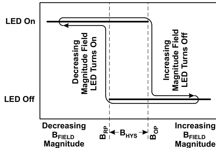
Figure 1: Hall Switch Control of LED State
