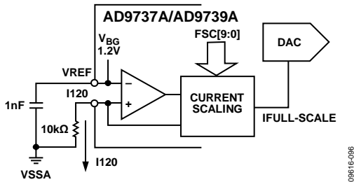
Figure 177. Voltage Reference Circuit
