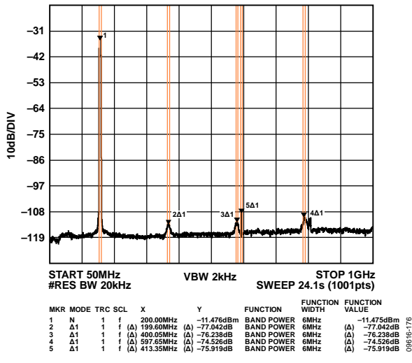
Figure 116. Low Band Wideband ACLR
