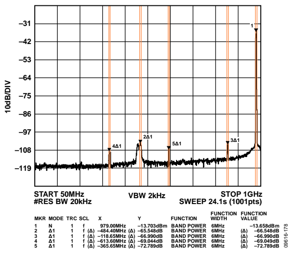
Figure 118. High Band Wideband ACLR
