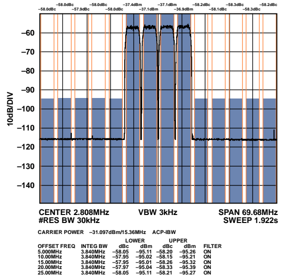
Figure 41. Typical Four-Carrier WCDMA ACLR Performance at 2.8 GHz, f_{DAC} = 2457.6 MSPS (Third Nyquist Zone)
