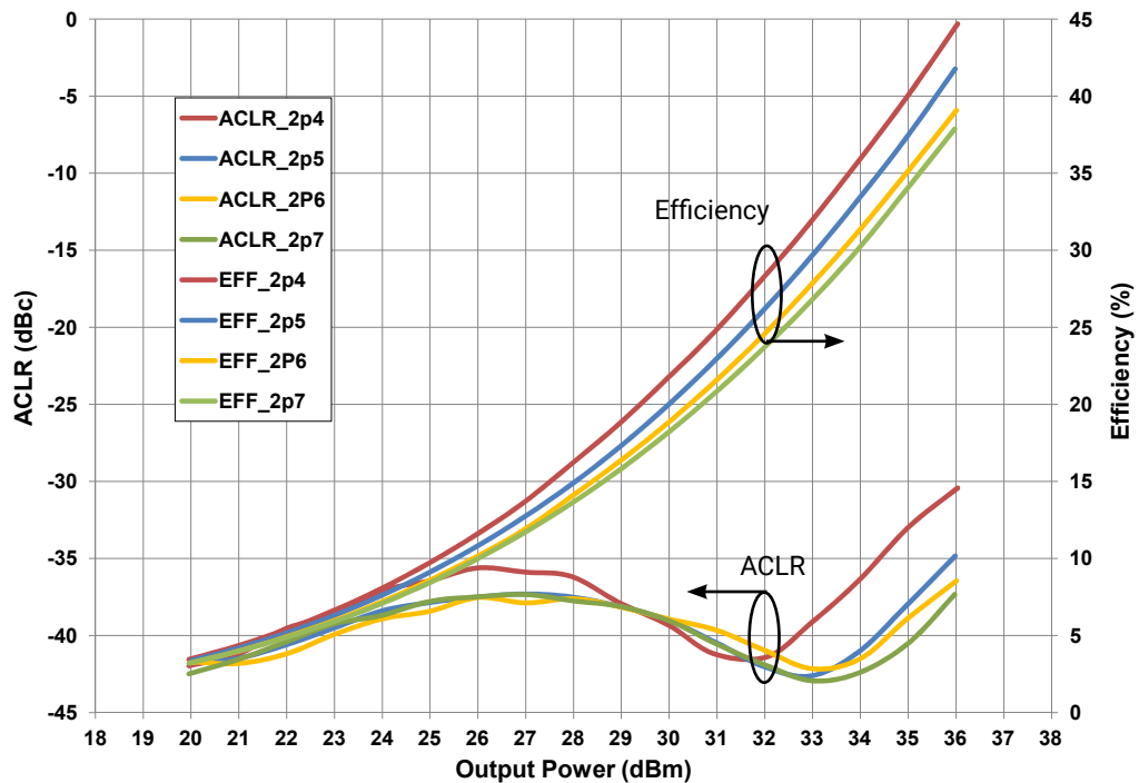
Figure 2. - Typical Drain Efficiency and ACLR vs. Output Power V_{DD} = 50\text{ V}, I_{DQ} = 60\text{ mA}, 1\text{ Carrier WCDMA}, \text{PAR} = 7.5\text{ dB}
